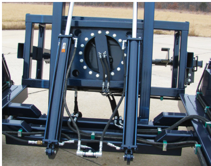
INTERNALLY RAN HYDRAULIC HOSES (NO HOSE DISCONNECT)
